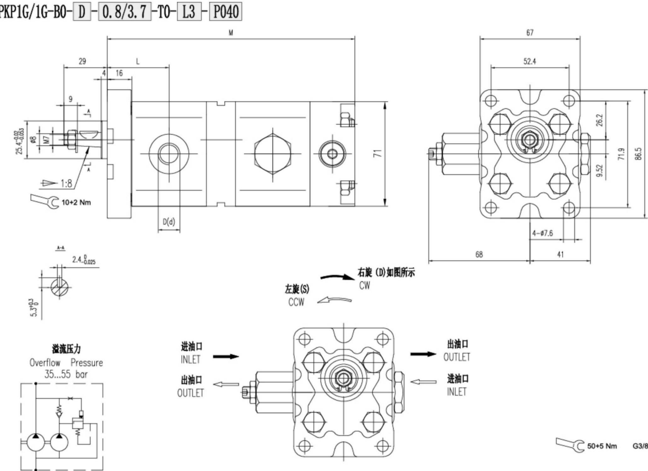
1G/1G高低压泵标准型产品尺寸/1G/1G High-Low Pump Standard Product Dimensions
